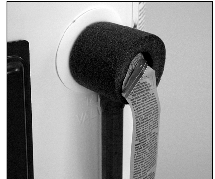
Make sure the insulation does not interfere with the T&P Relief Valve's operation.
