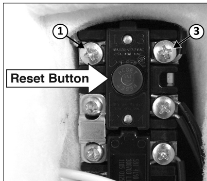
Energy Cut Off (ECO) button
